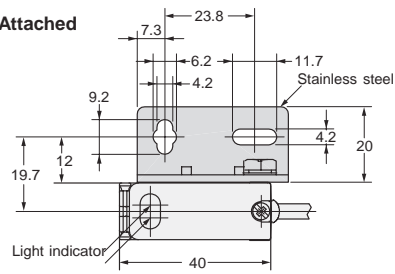
Mounting Holes
